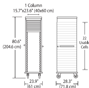
FHLMS80-TSKL Tambour Door Cart Wt: 285 Lb. Cart Dim: 23.9"W x 28.3"D x 80.6"H
