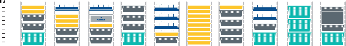
42.7" (106.7 cm) Half Height Carts 9 Cells
