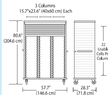
FH2653 Tambour Door Cart Wt: 500 Lb. Cart Dim: 57.7"W x 28.3"D x 80.6"H
