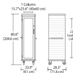
FHLMS80-LGKL Glass Door with Left Hinge FHLMS80-RGKL Glass Door with Right Hinge Cart Wt: 295 Lb. Cart Dim: 23.9"W x 28.3"D x 80.6"H
