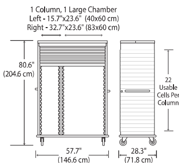
FH2653LC Tambour Door Cart Wt: 490 Lb. Cart Dim: 57.7"W x 28.3"D x 80.6"H
