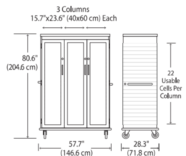
FH2653HG Glass Doors Cart Wt: 530 Lb. Cart Dim: 57.7"W x 28.3"D x 80.6"H
