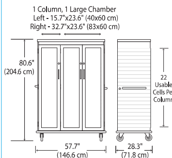
FH2653LCHG Glass Doors Cart Wt: 510 Lb. Cart Dim: 57.7"W x 28.3"D x 80.6"H
